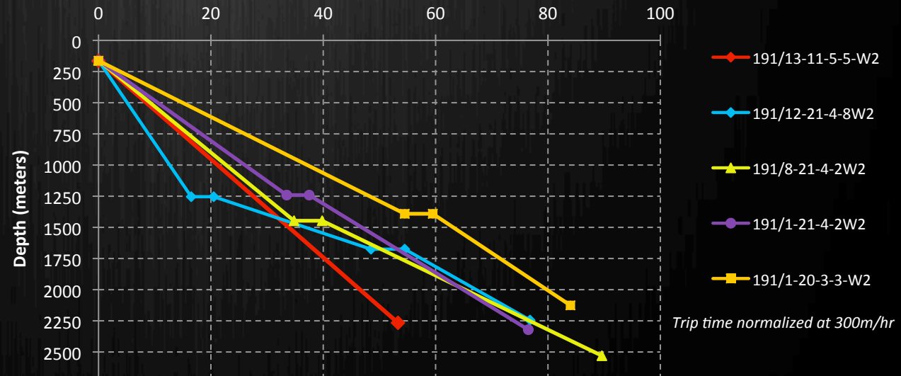
DRLG Curve Comparison Cumulative DRLG Hrs
