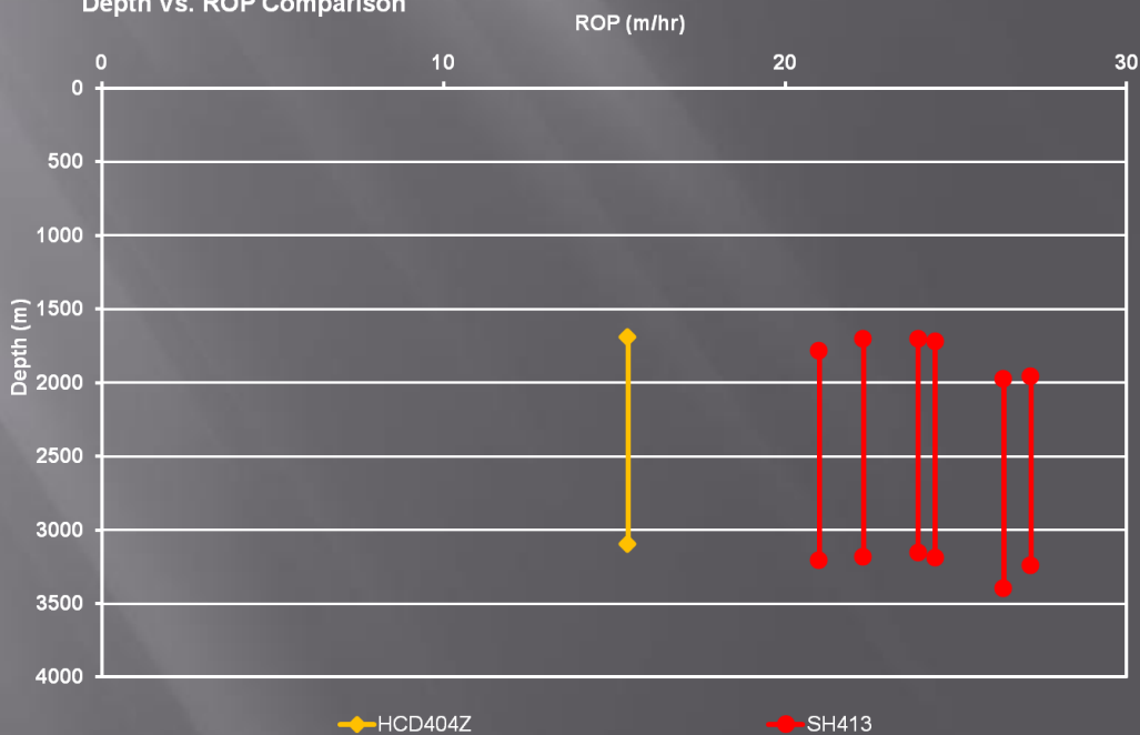
Depth Vs. ROP Comparison
